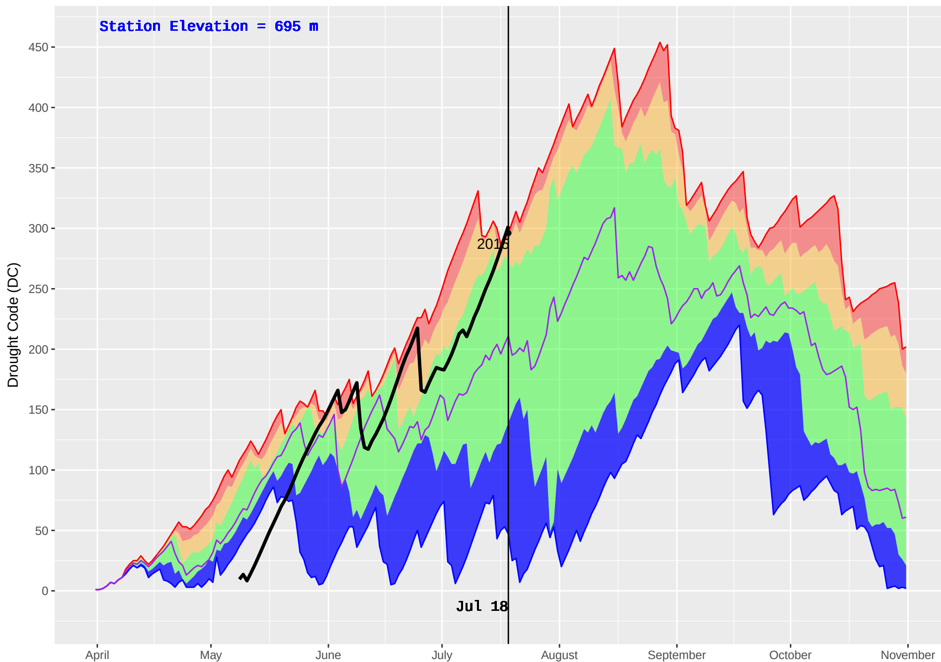
BLUE RIVER 2 (1108) : Historical (2011–2016) and Current (2018) Daily Drought Code (DC)
