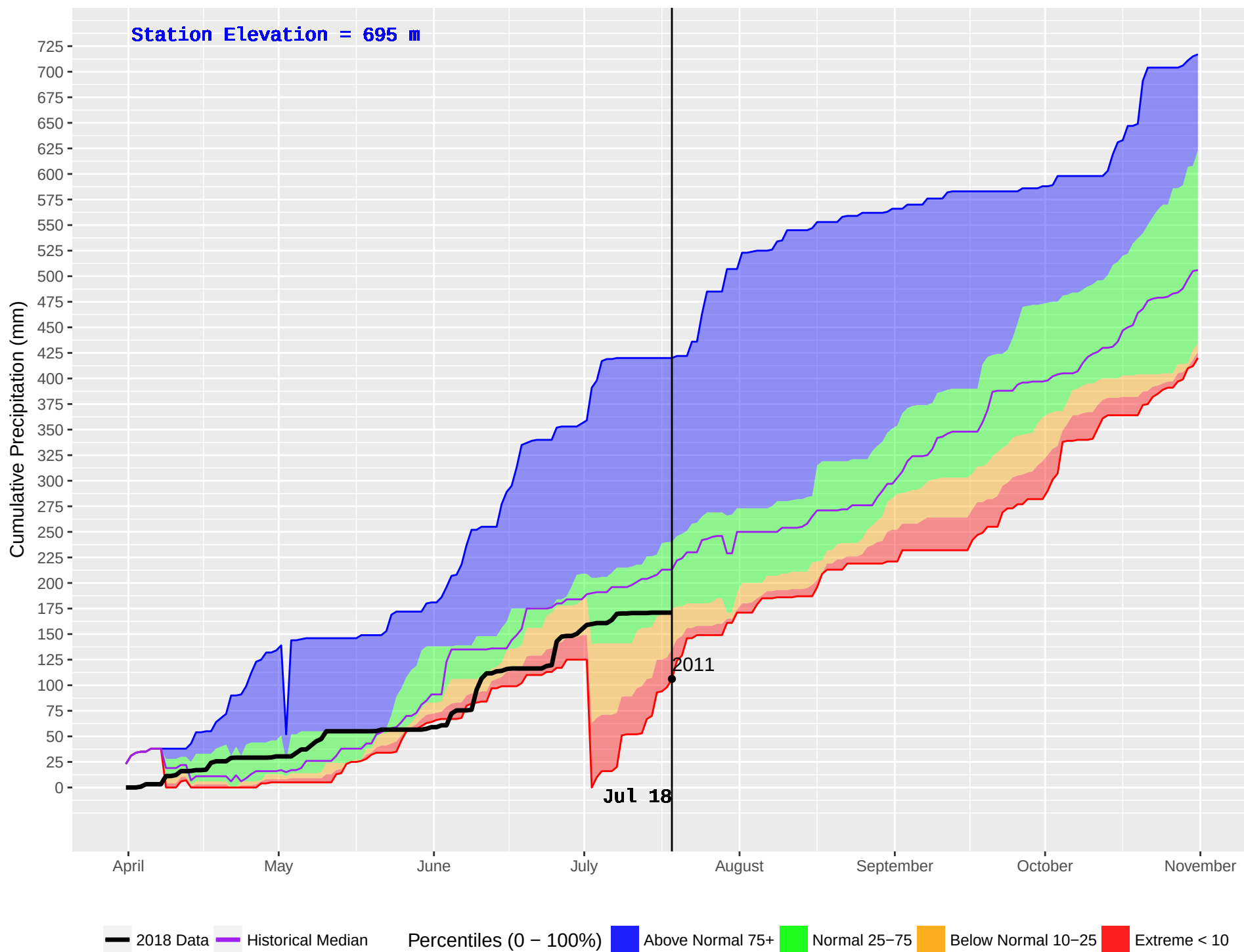
BLUE RIVER 2 (1108) : Historical (2011–2016) and Current (2018) Daily Cumulative Precipitation
