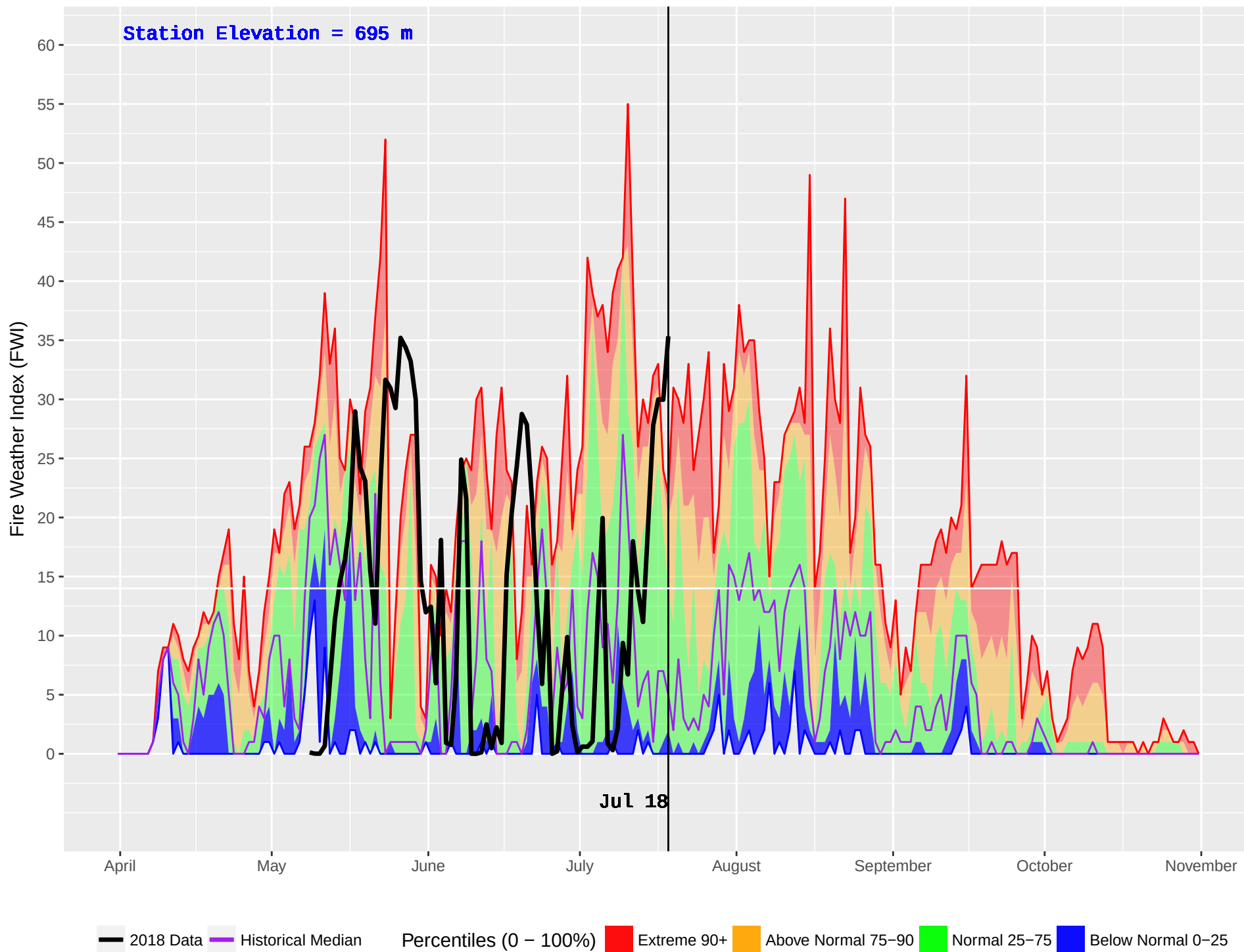
BLUE RIVER 2 (1108) : Historical (2011–2016) and Current (2018) Daily Fire Weather Index (FWI)
